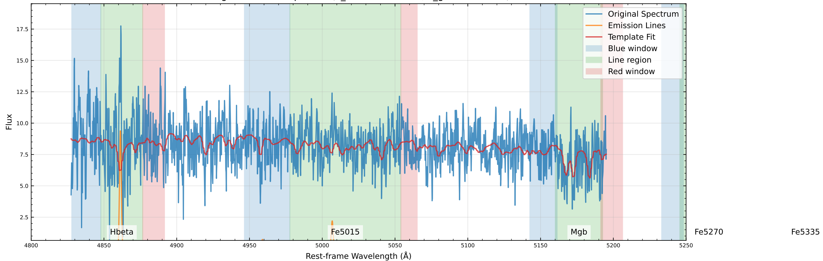
Original Data Comparison (v_star=-15.3 km/s, v_gas=-9.7 km/s)
