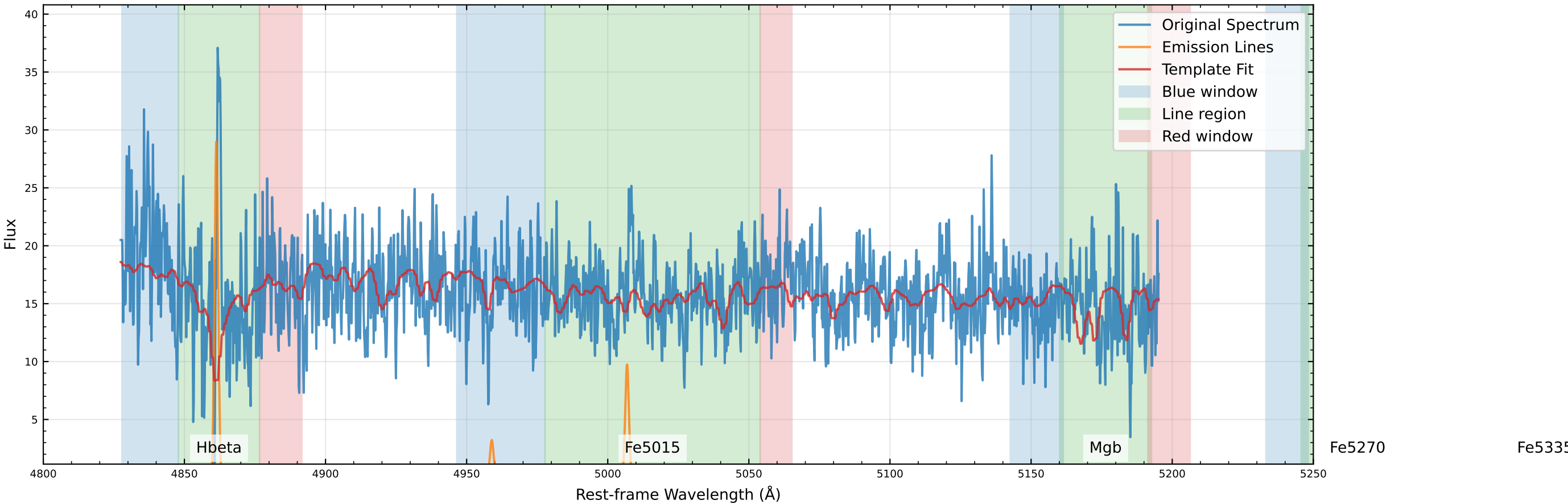
Original Data Comparison (v_star=77.1 km/s, v_gas=58.8 km/s)
