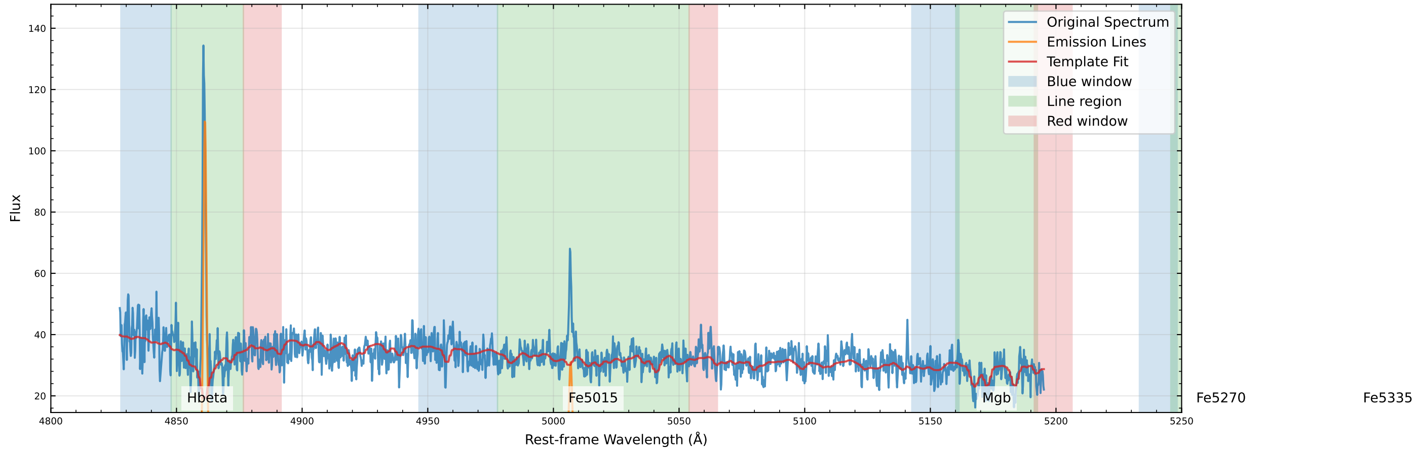
Original Data Comparison (v_star=4.5 km/s, v_gas=-22.9 km/s)
