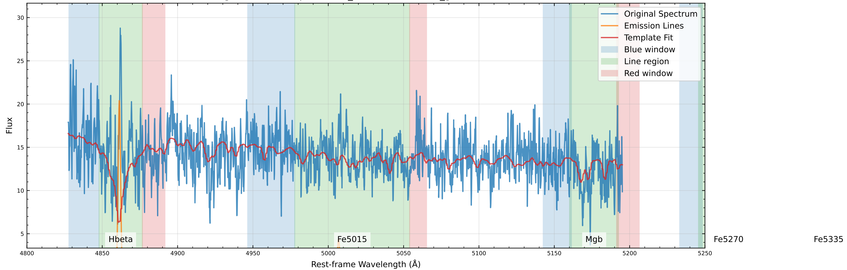
Original Data Comparison (v_star=59.1 km/s, v_gas=48.1 km/s)
