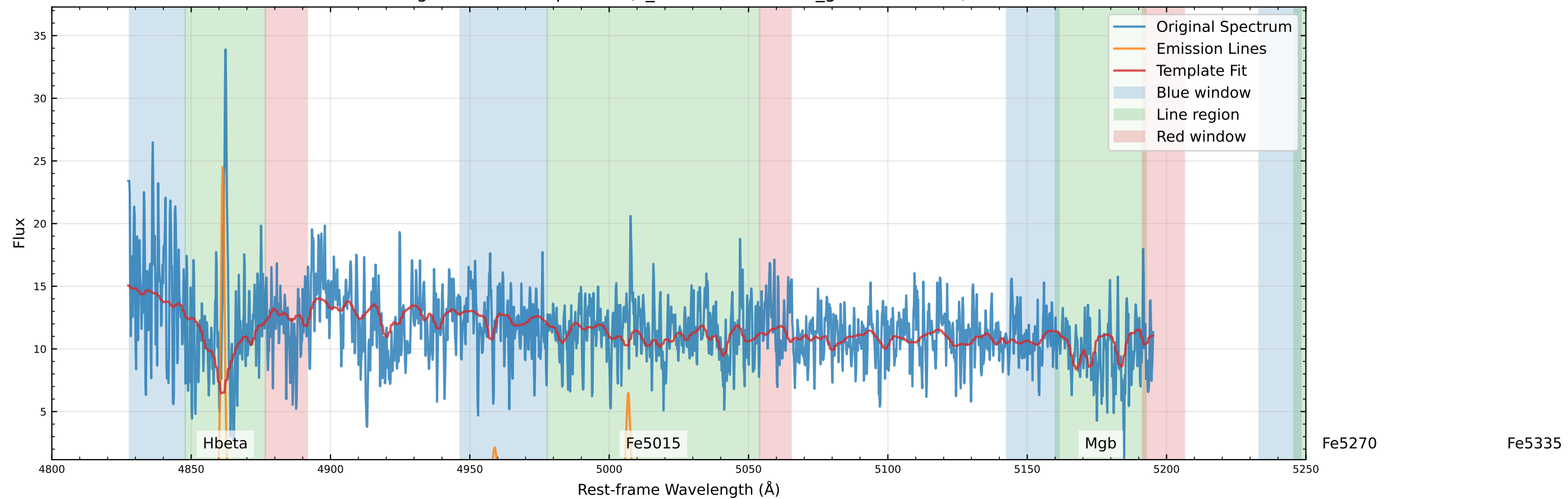
Original Data Comparison (v_star=59.6 km/s, v_gas=59.0 km/s)
