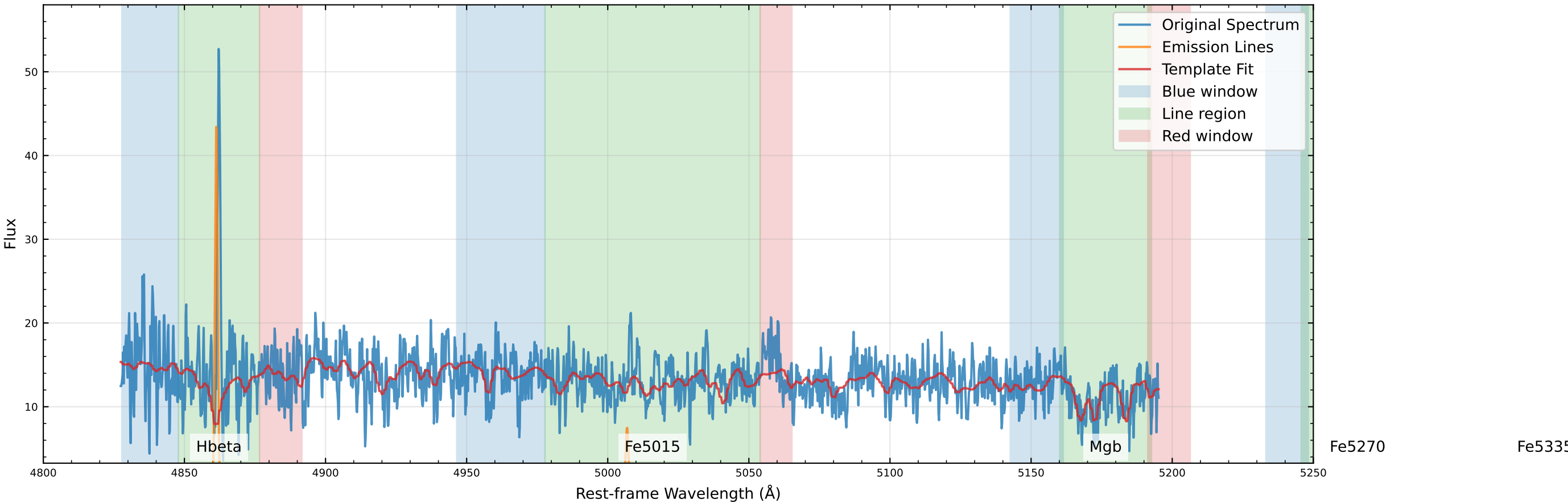
Original Data Comparison (v_star=48.8 km/s, v_gas=55.3 km/s)
