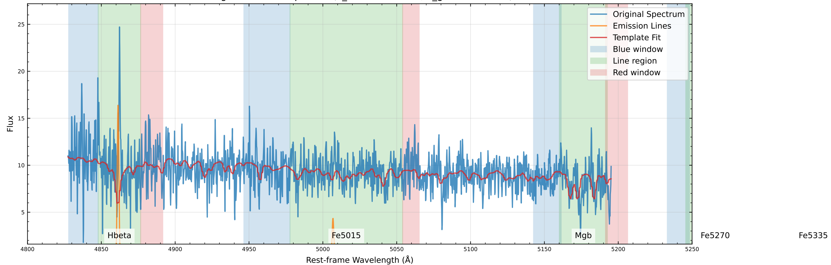
Original Data Comparison (v_star=69.8 km/s, v_gas=60.5 km/s)
