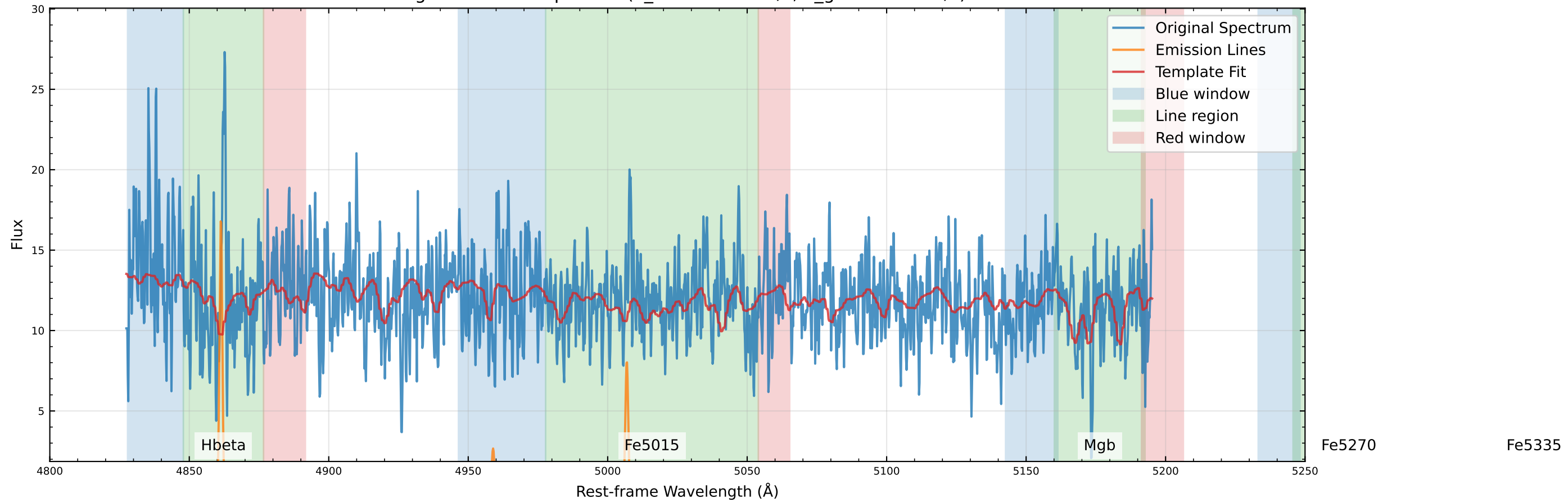
Original Data Comparison (v_star=67.1 km/s, v_gas=69.0 km/s)
