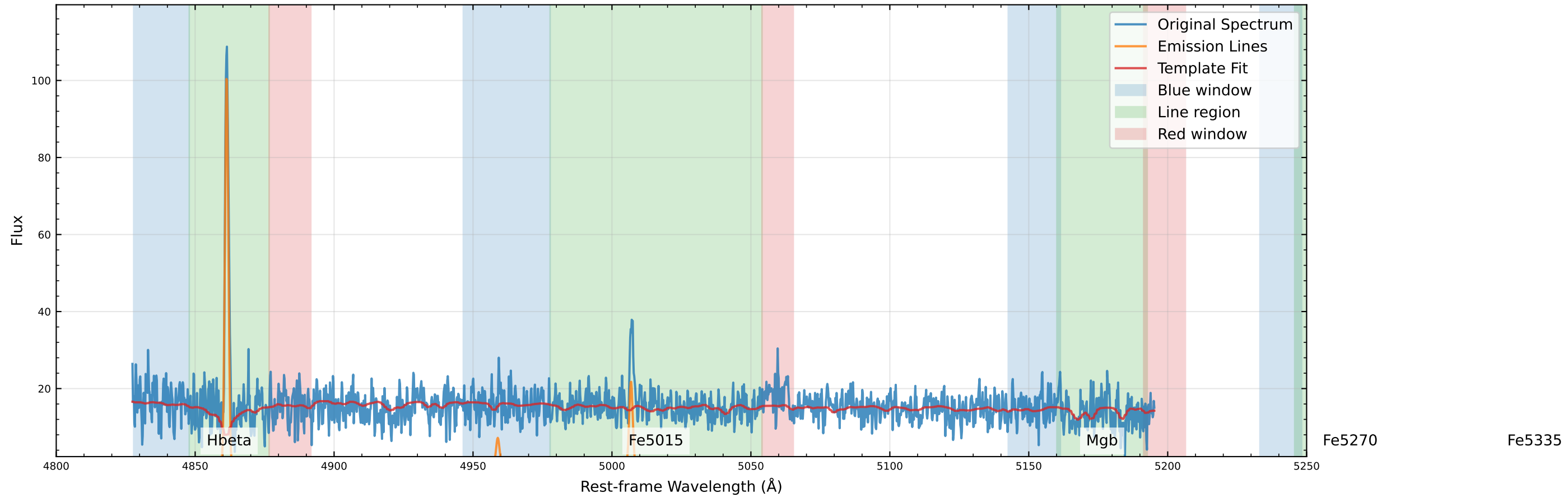
Original Data Comparison (v_star=0.4 km/s, v_gas=5.1 km/s)
