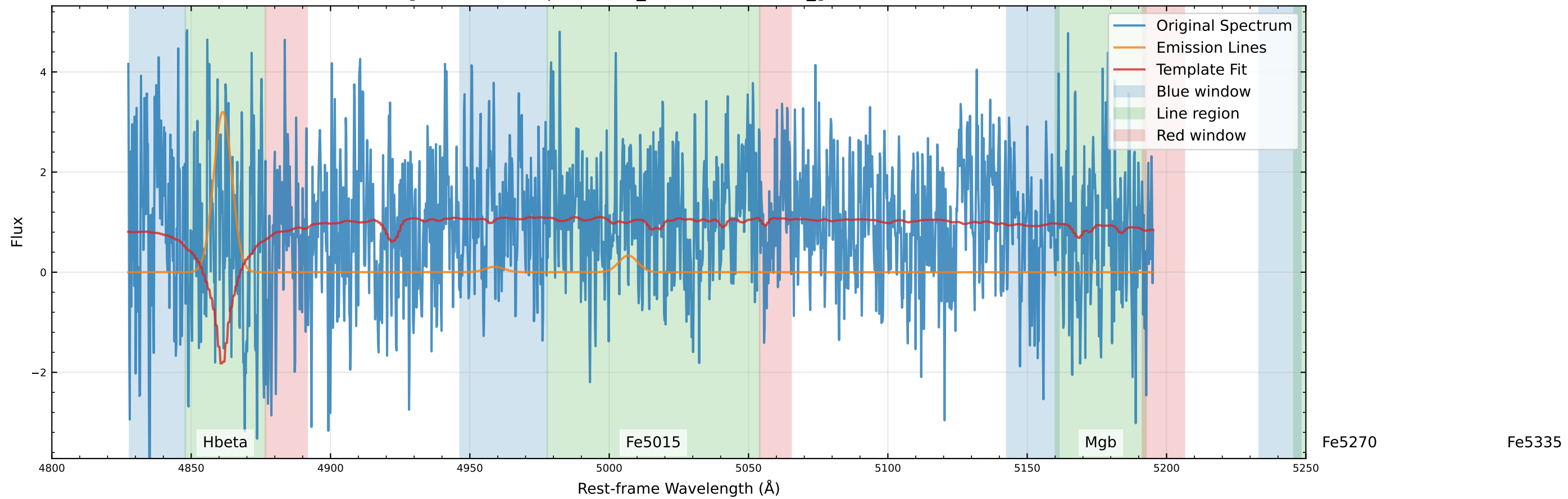
Original Data Comparison (v_star=23.0 km/s, v_gas=-159.2 km/s)
