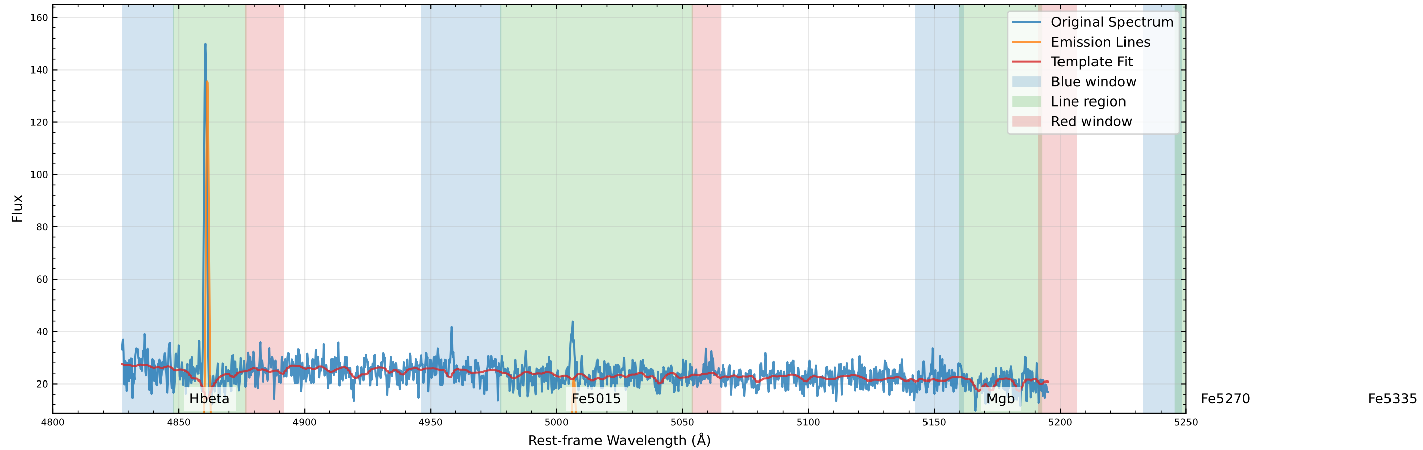
Original Data Comparison (v_star=-49.4 km/s, v_gas=-49.1 km/s)
