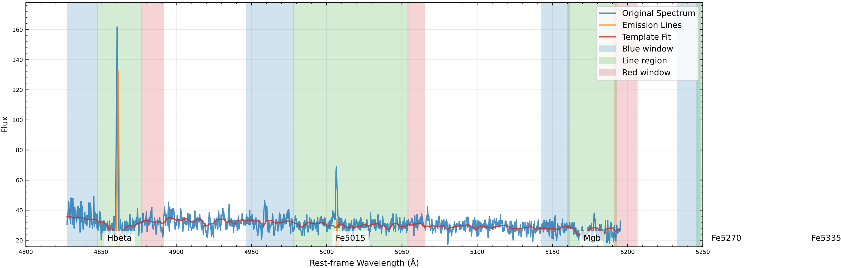
Original Data Comparison (v_star=-9.4 km/s, v_gas=-38.7 km/s)
