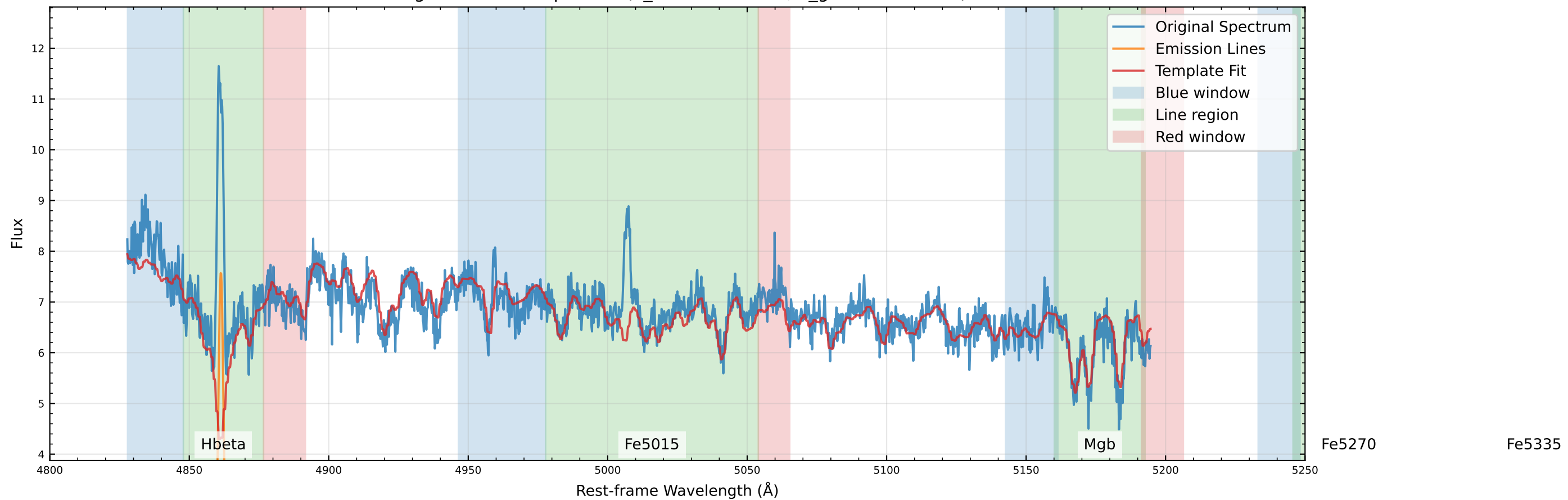
Original Data Comparison (v_star=-5.3 km/s, v_gas=-14.3 km/s)
