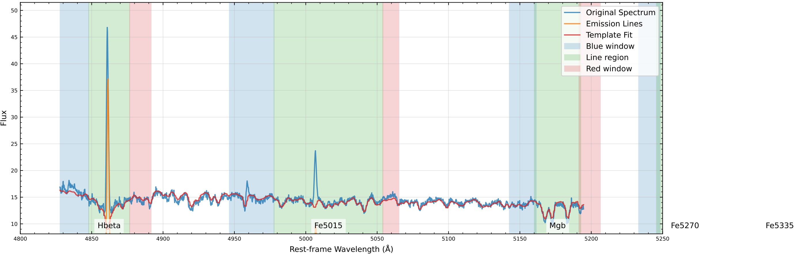
Original Data Comparison (v_star=-4.5 km/s, v_gas=-20.7 km/s)
