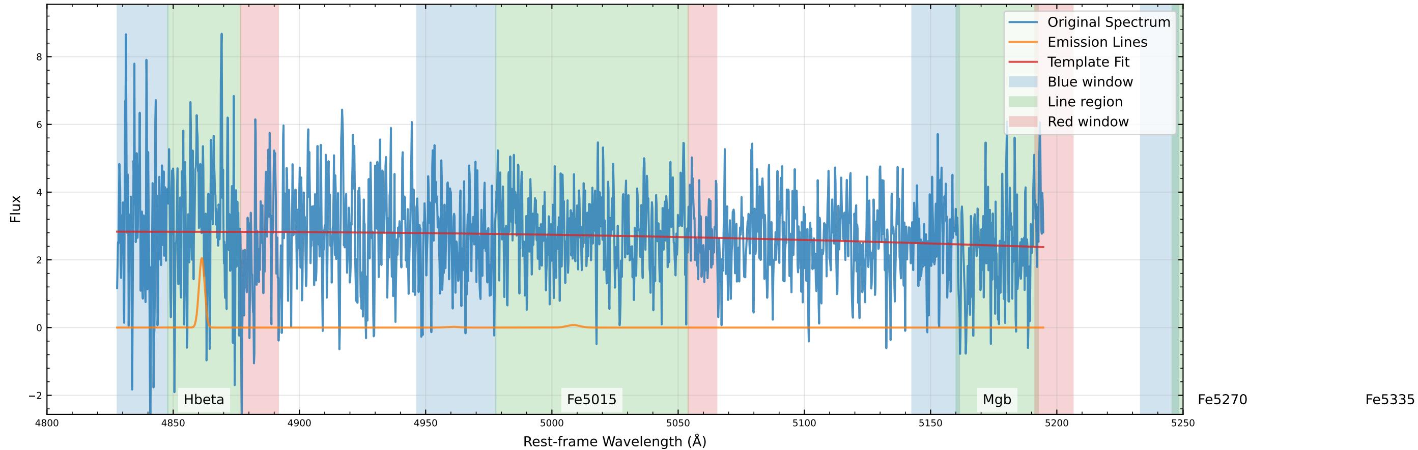
Original Data Comparison (v_star=-46.2 km/s, v_gas=-113.4 km/s)
