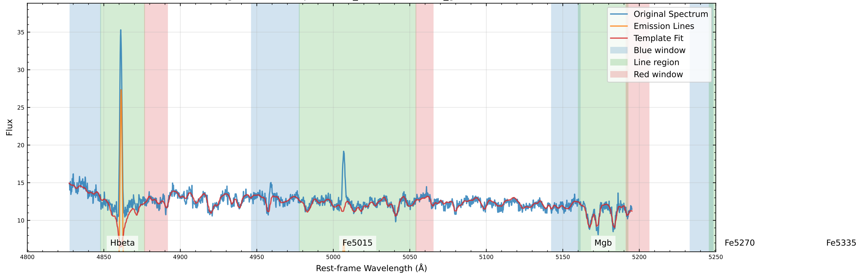
Original Data Comparison (v_star=-6.1 km/s, v_gas=-10.7 km/s)
