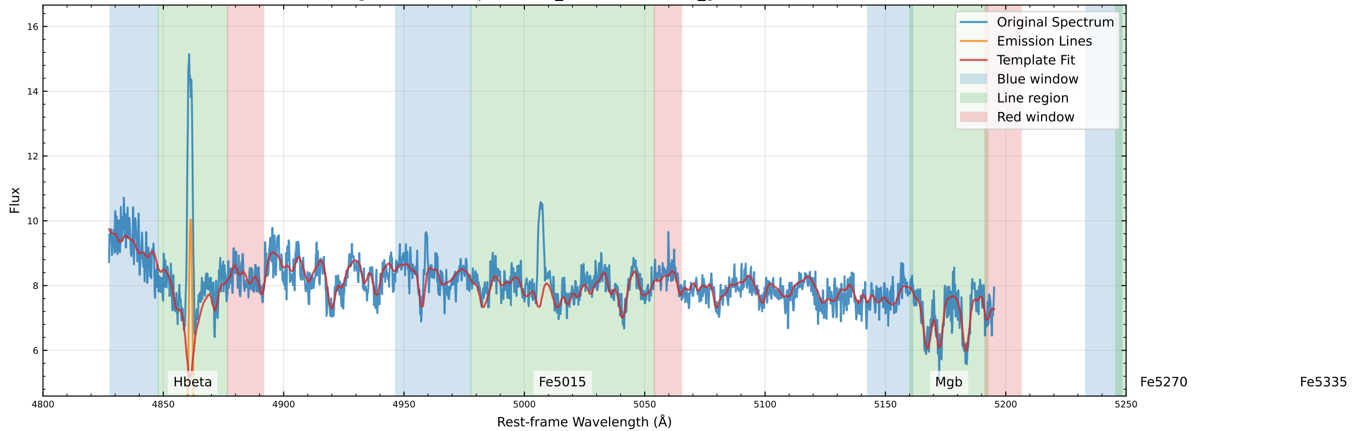
Original Data Comparison (v_star=-9.2 km/s, v_gas=-16.2 km/s)
