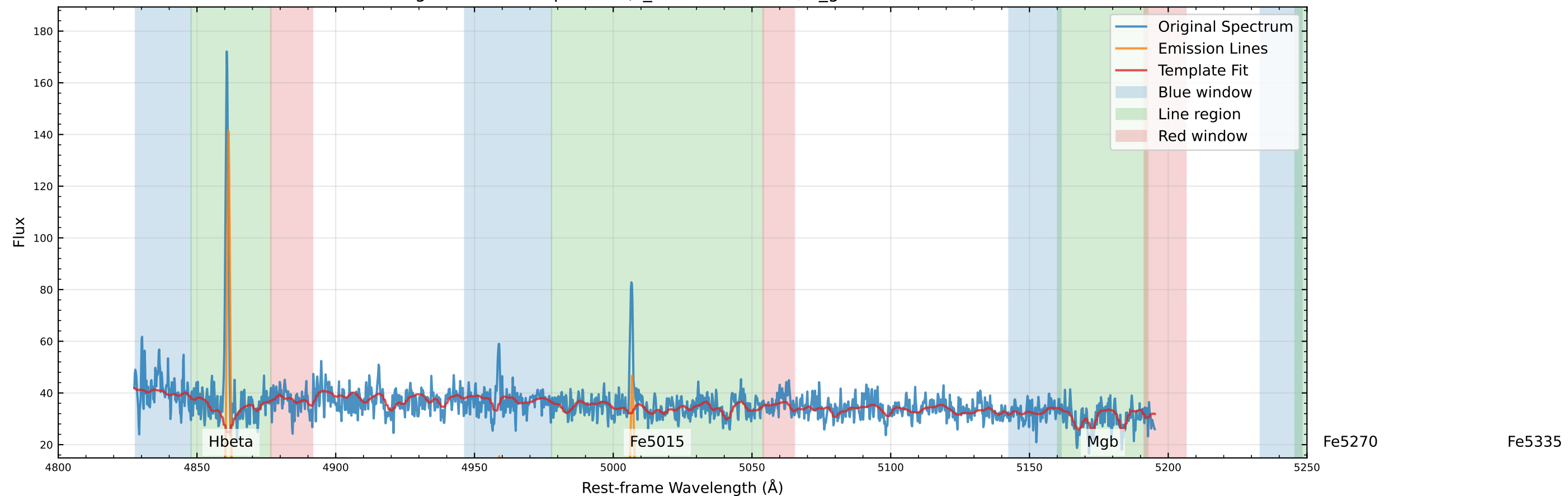
Original Data Comparison (v_star=-16.4 km/s, v_gas=-33.3 km/s)
