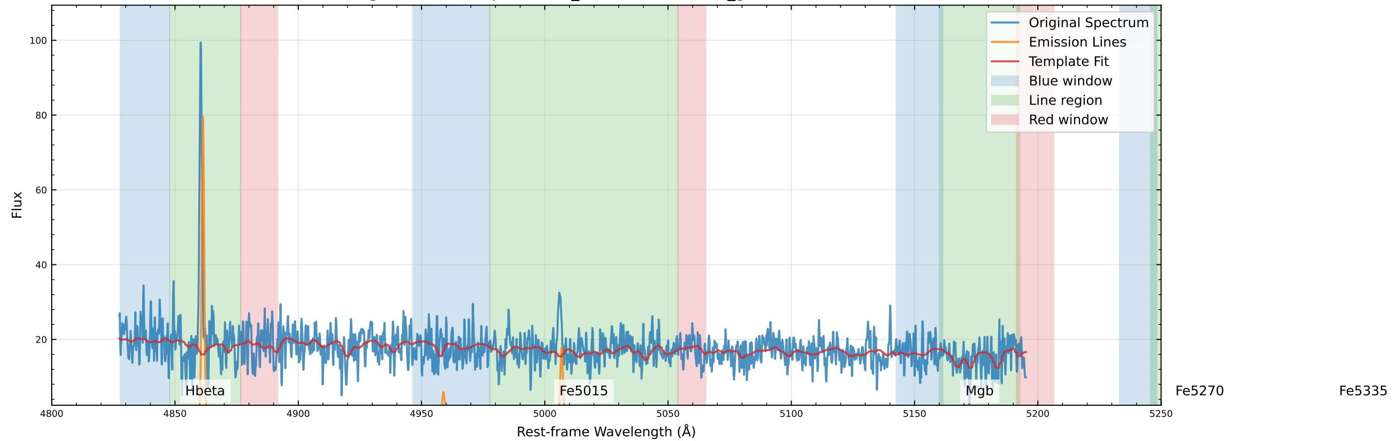
Original Data Comparison (v_star=-54.7 km/s, v_gas=-55.8 km/s)
