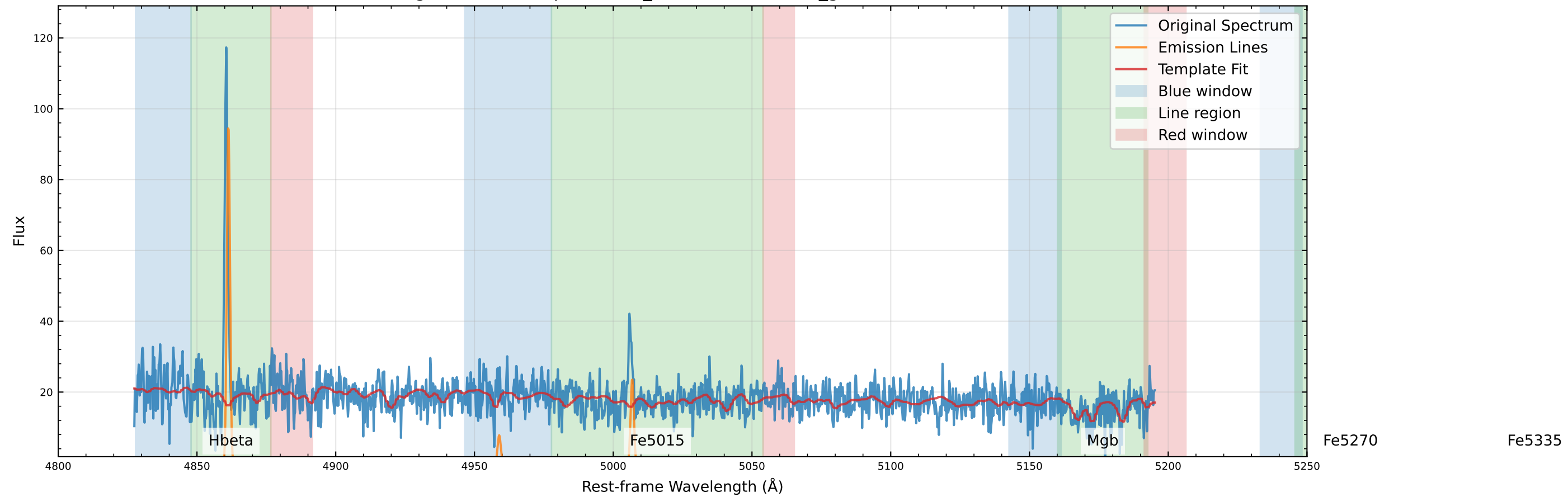
Original Data Comparison (v_star=-40.4 km/s, v_gas=-49.2 km/s)
