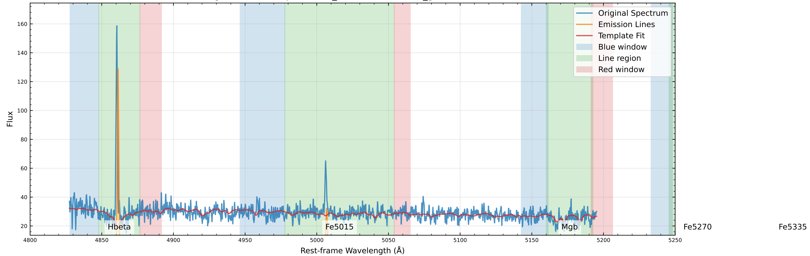
Original Data Comparison (v_star=-34.7 km/s, v_gas=-52.4 km/s)
