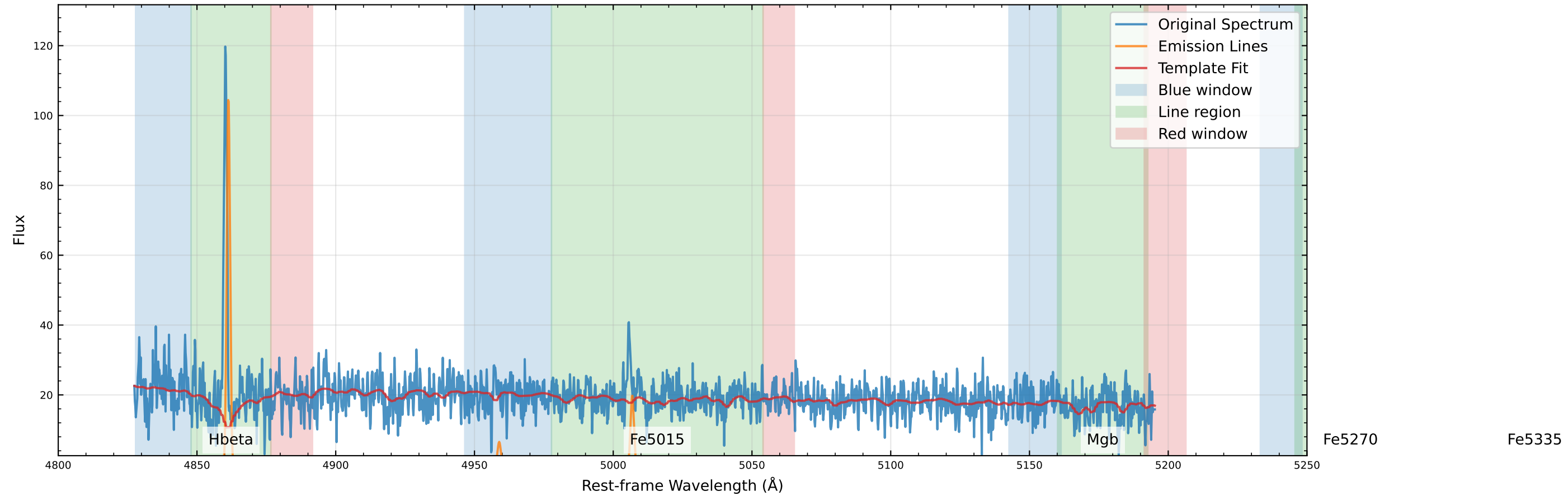
Original Data Comparison (v_star=-69.1 km/s, v_gas=-66.8 km/s)
