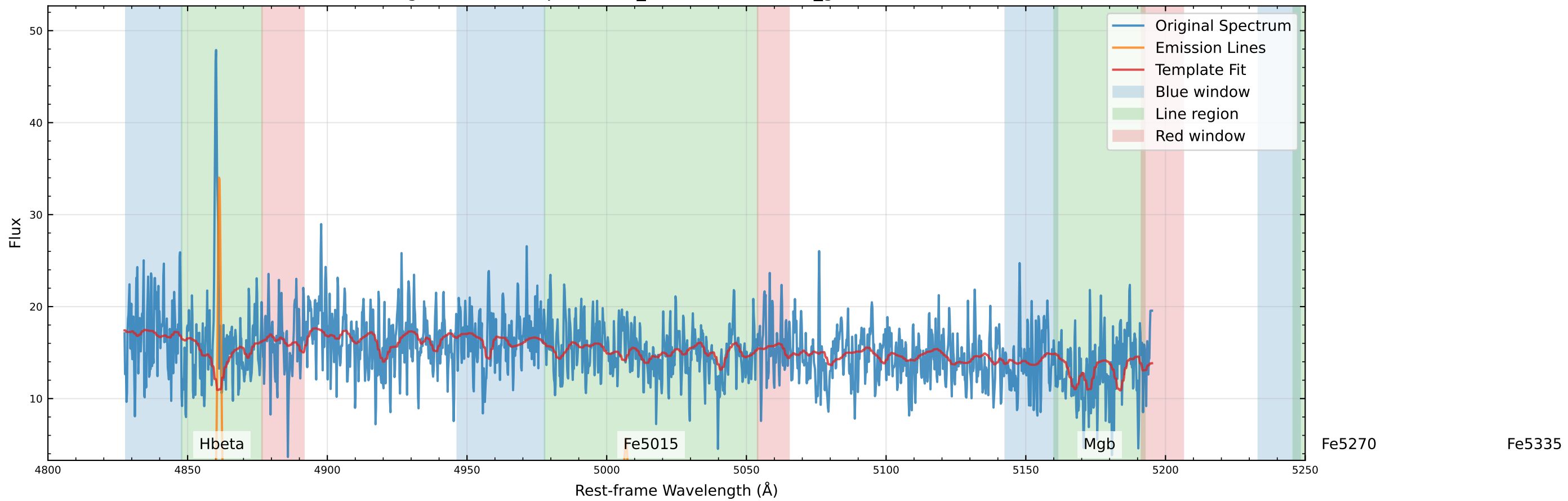
Original Data Comparison (v_star=-81.6 km/s, v_gas=-71.1 km/s)
