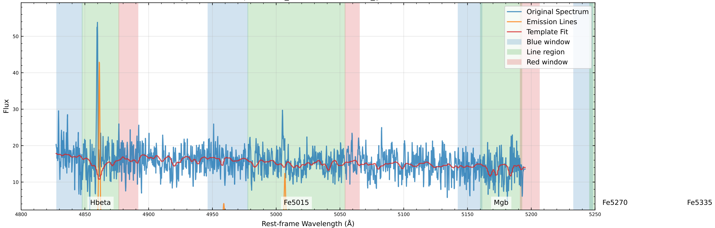
Original Data Comparison (v_star=-137.5 km/s, v_gas=-104.3 km/s)
