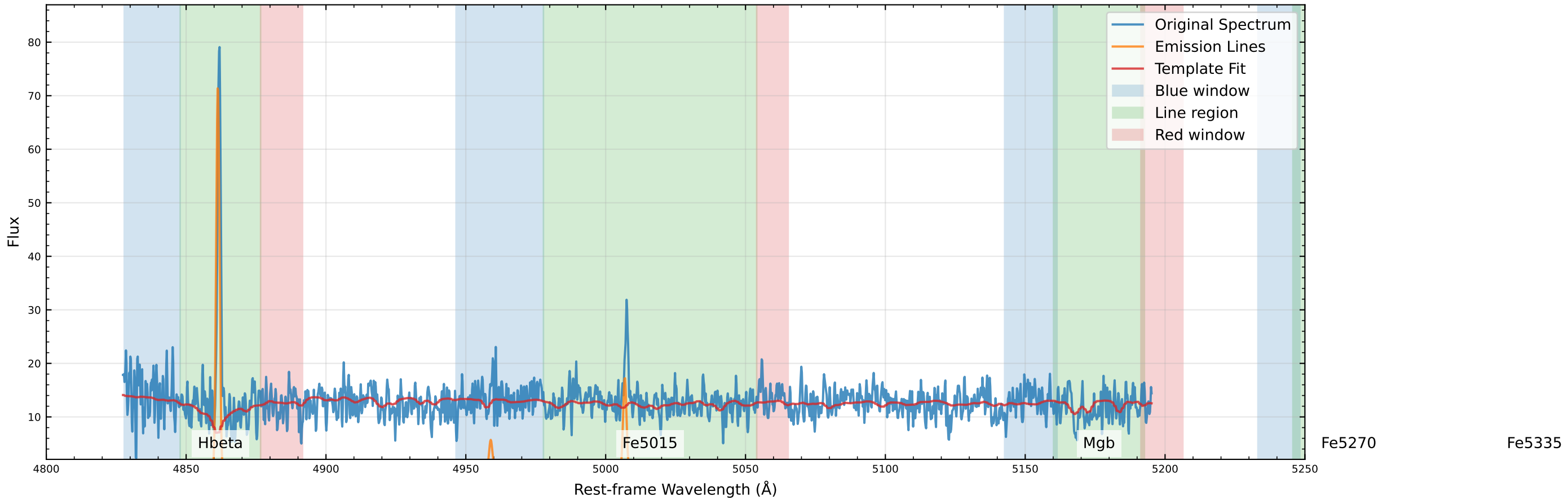
Original Data Comparison (v_star=49.5 km/s, v_gas=29.3 km/s)
