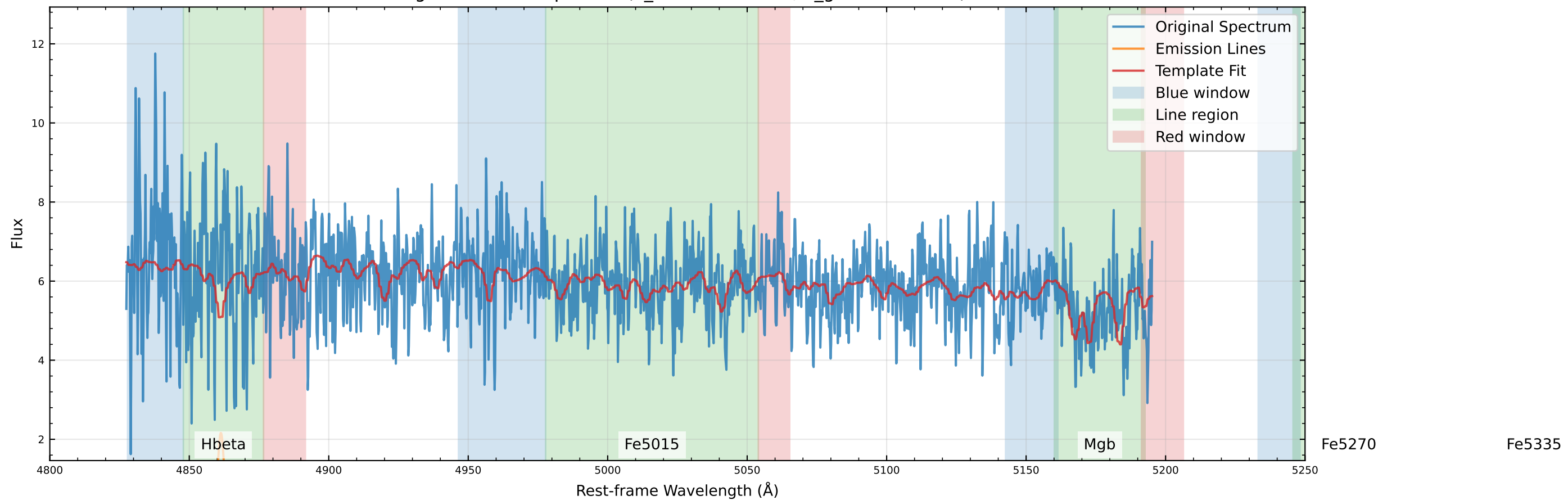
Original Data Comparison (v_star=82.0 km/s, v_gas=91.3 km/s)
