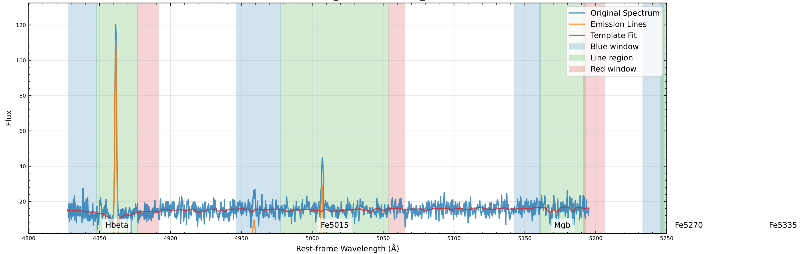
Original Data Comparison (v_star=37.9 km/s, v_gas=5.2 km/s)
