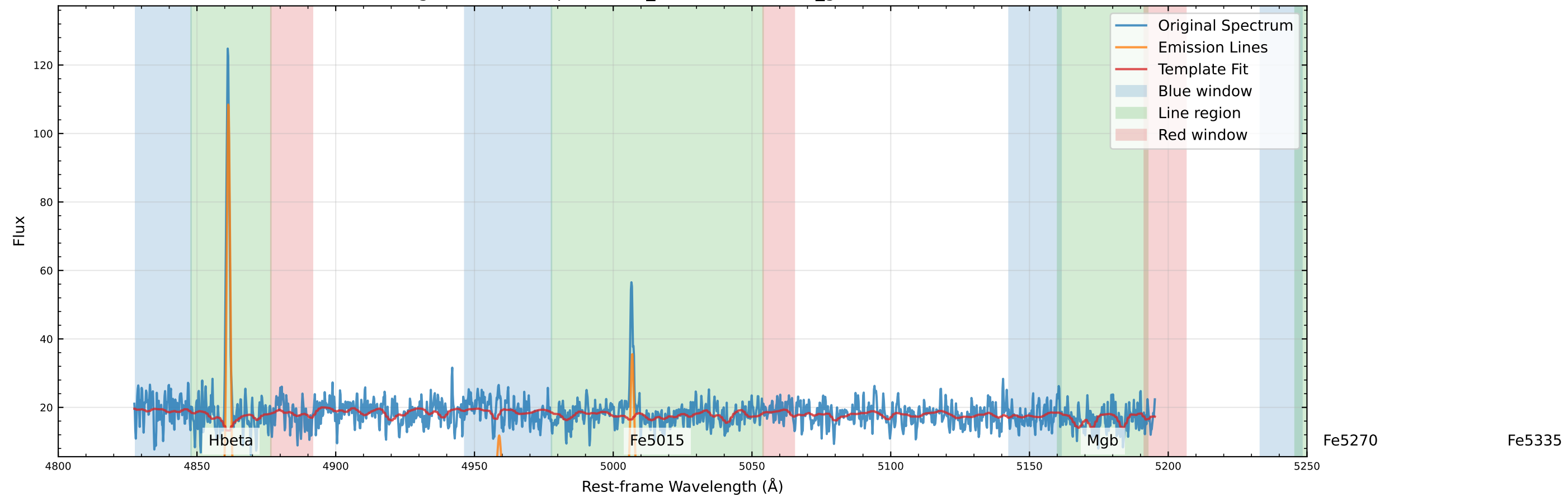
Original Data Comparison (v_star=12.1 km/s, v_gas=-13.0 km/s)
