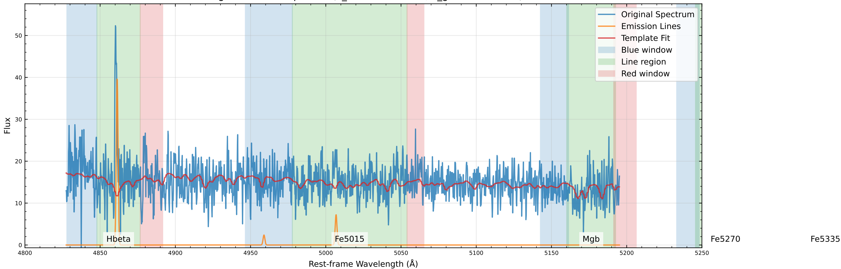
Original Data Comparison (v_star=-29.6 km/s, v_gas=-53.6 km/s)
