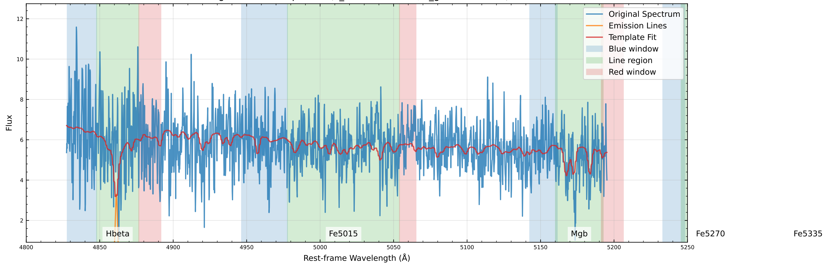
Original Data Comparison (v_star=45.2 km/s, v_gas=16.9 km/s)
