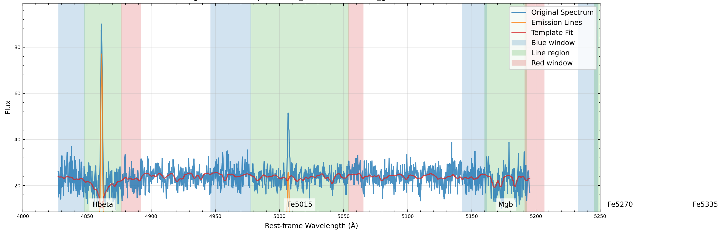
Original Data Comparison (v_star=22.9 km/s, v_gas=0.1 km/s)
