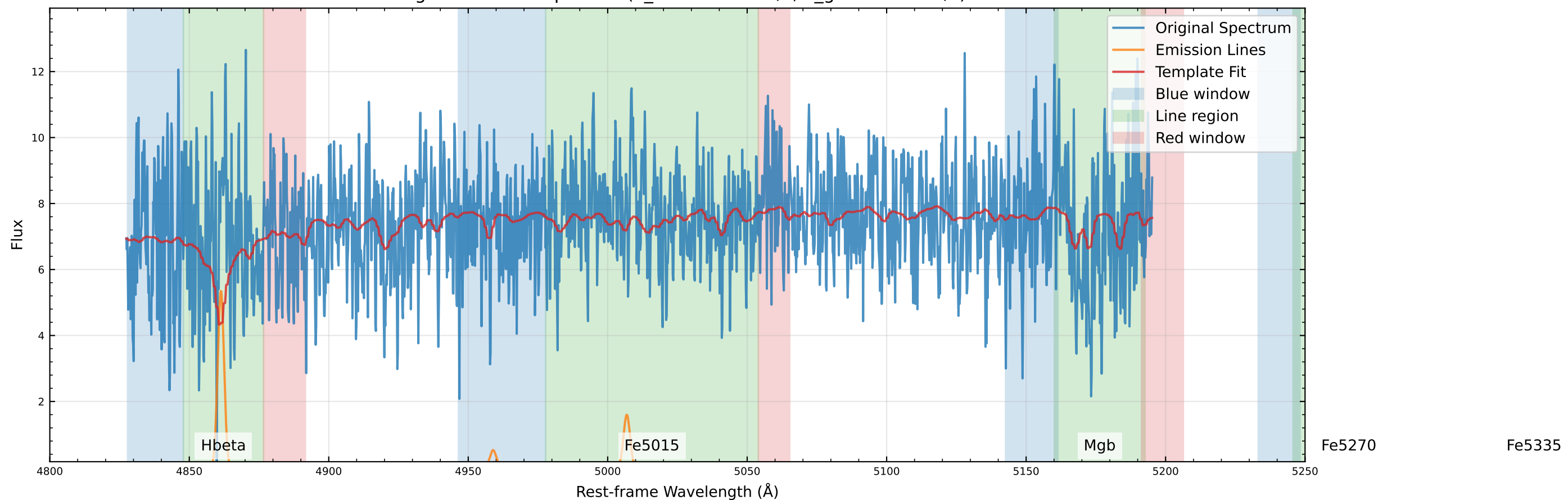
Original Data Comparison (v_star=55.5 km/s, v_gas=64.7 km/s)
