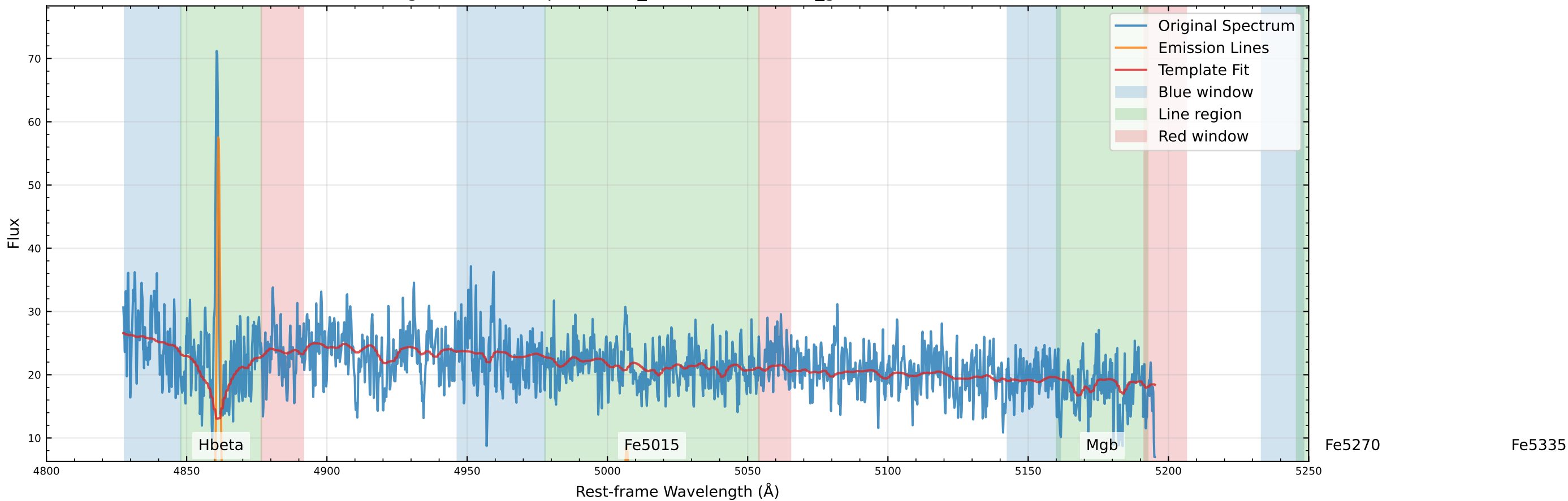
Original Data Comparison (v_star=-37.0 km/s, v_gas=-33.9 km/s)
