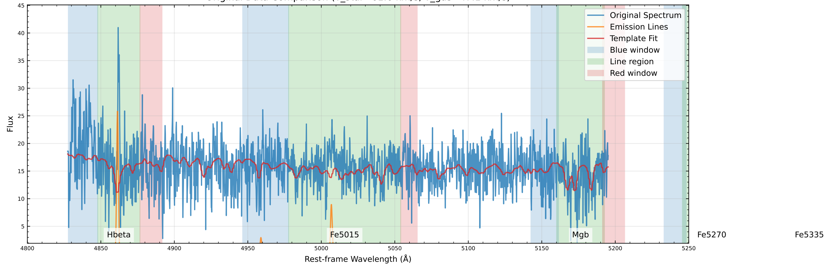
Original Data Comparison (v_star=61.6 km/s, v_gas=47.1 km/s)
