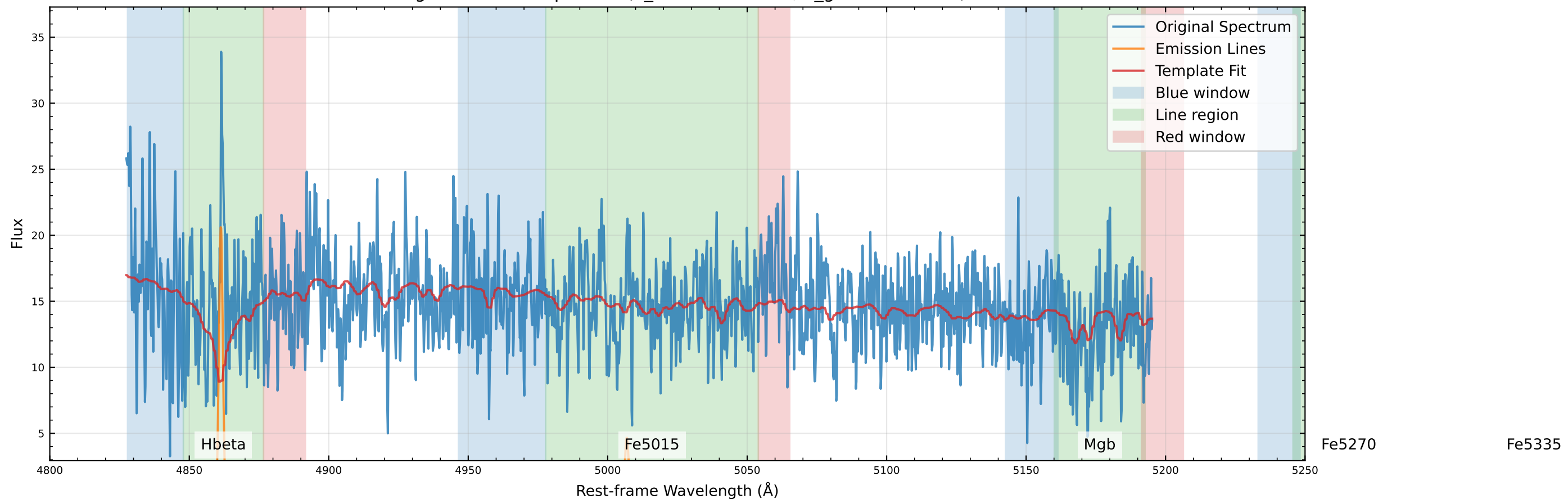
Original Data Comparison (v_star=12.1 km/s, v_gas=25.3 km/s)
