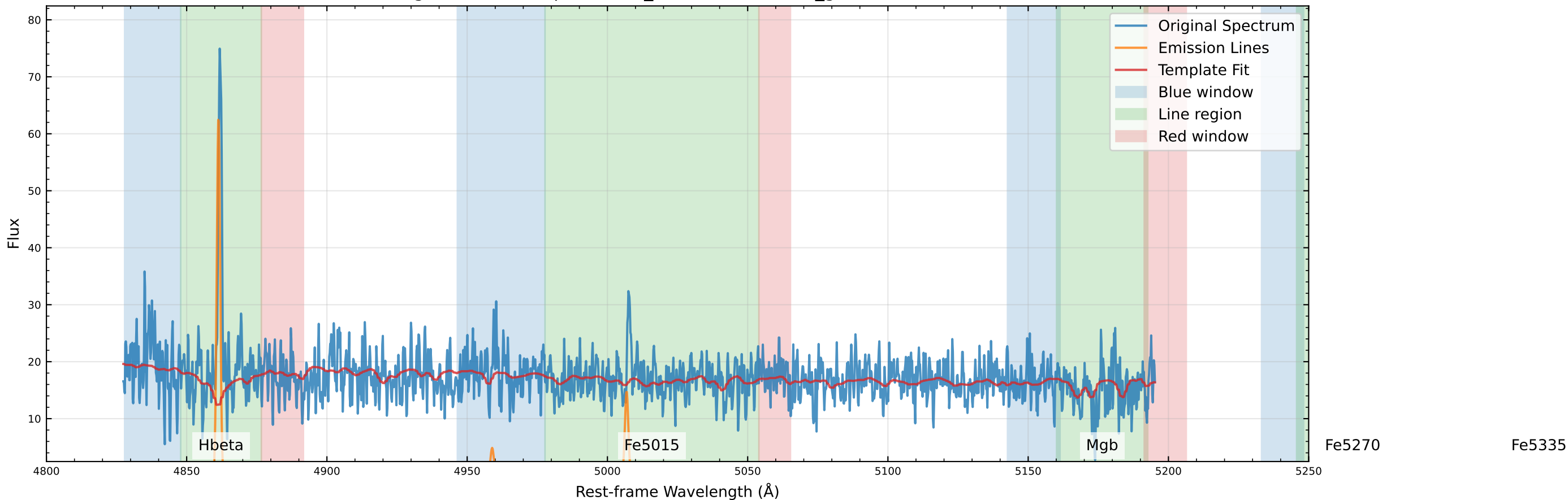
Original Data Comparison (v_star=34.9 km/s, v_gas=36.1 km/s)
