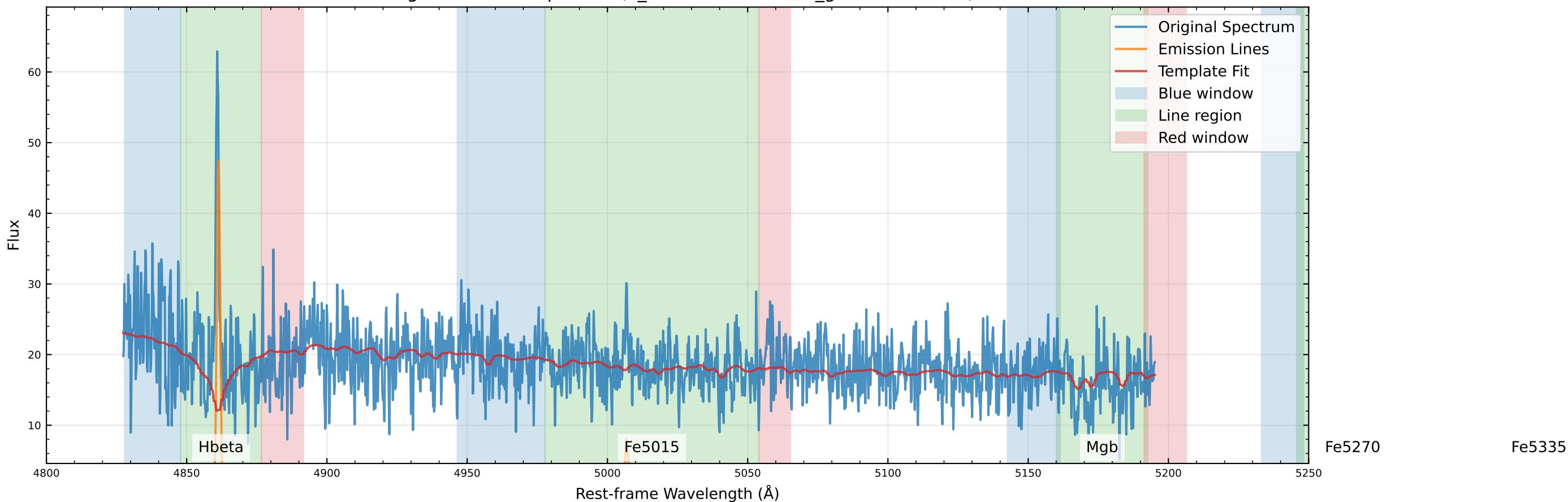
Original Data Comparison (v_star=-23.8 km/s, v_gas=-25.7 km/s)
