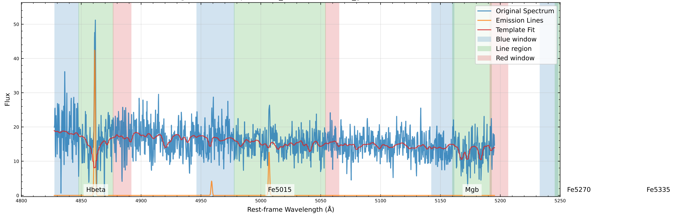
Original Data Comparison (v_star=29.4 km/s, v_gas=6.8 km/s)
