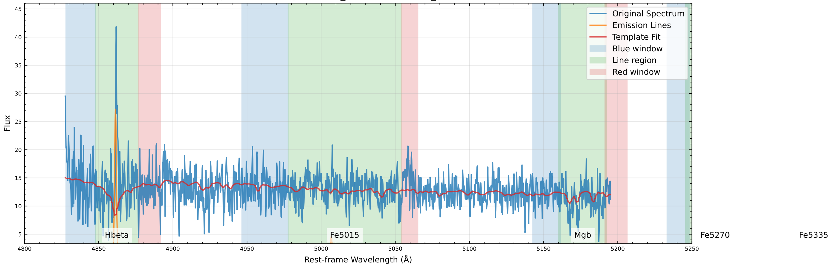
Original Data Comparison (v_star=32.7 km/s, v_gas=41.2 km/s)
