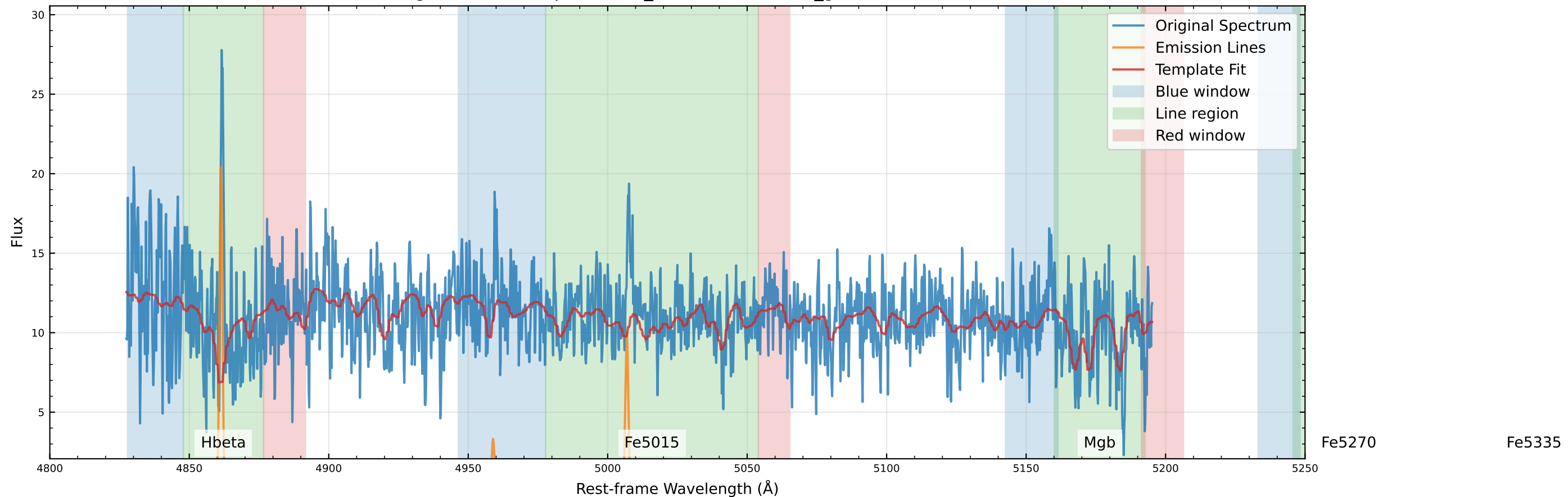
Original Data Comparison (v_star=35.9 km/s, v_gas=30.9 km/s)
