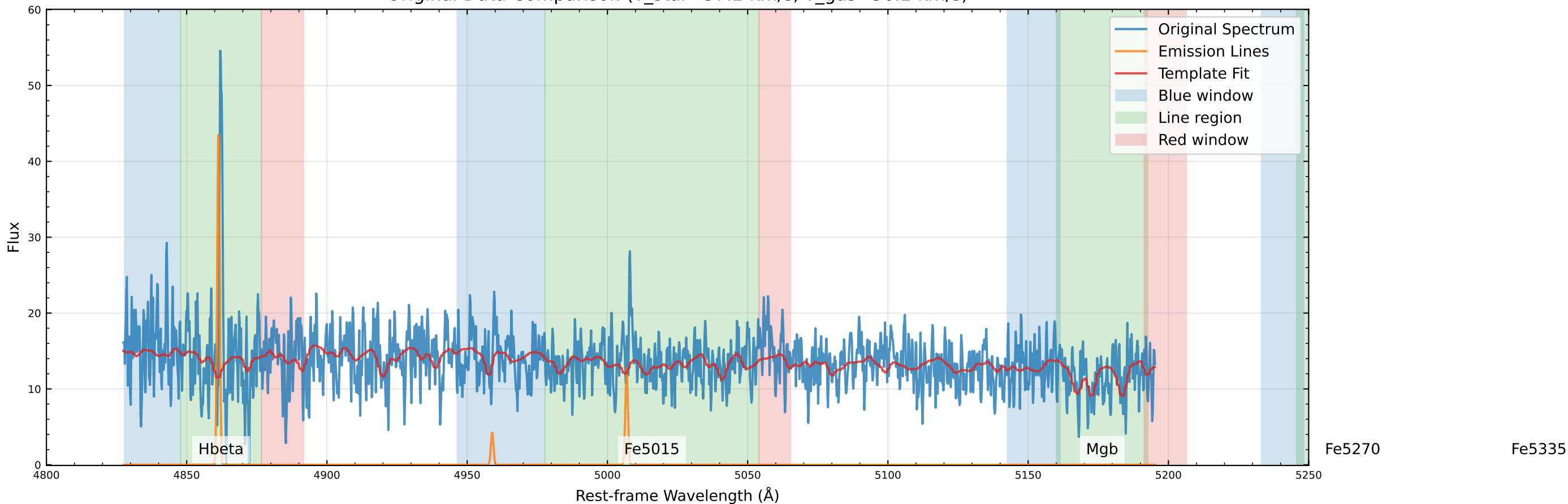
Original Data Comparison (v_star=57.2 km/s, v_gas=56.2 km/s)
