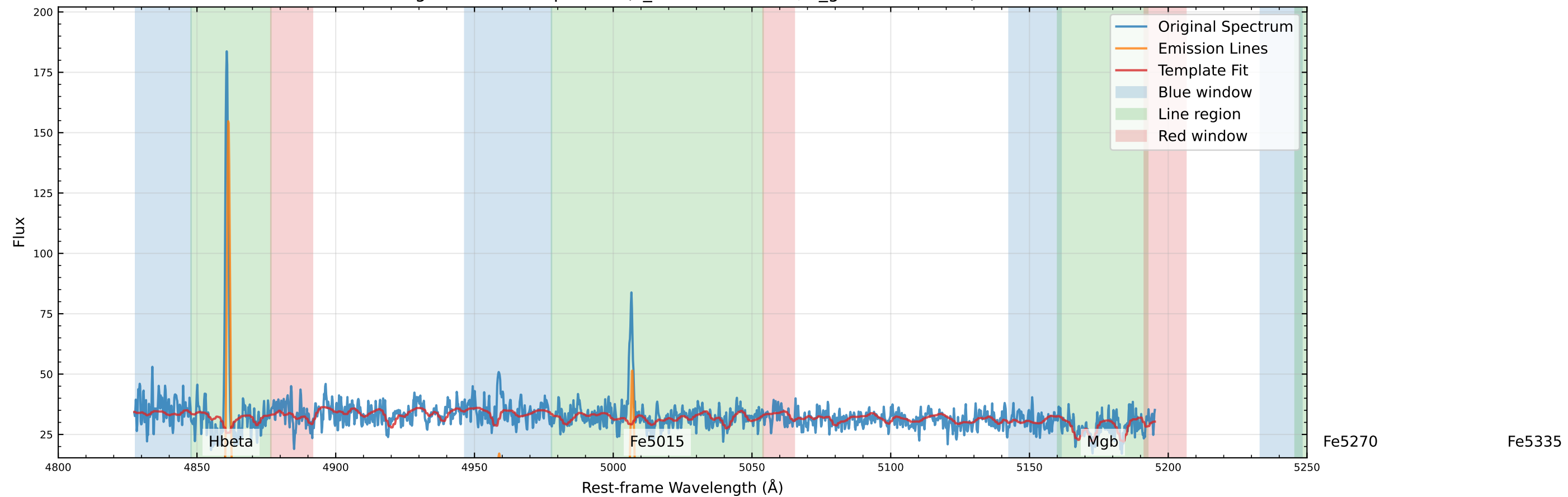
Original Data Comparison (v_star=-17.4 km/s, v_gas=-34.9 km/s)
