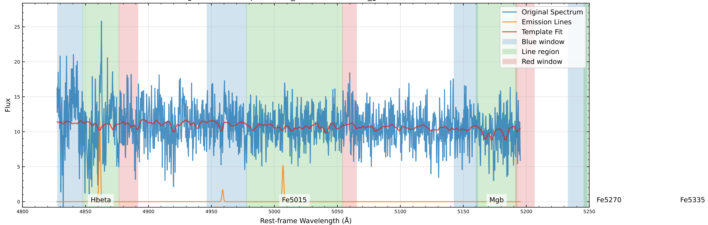
Original Data Comparison (v_star=45.0 km/s, v_gas=64.0 km/s)
