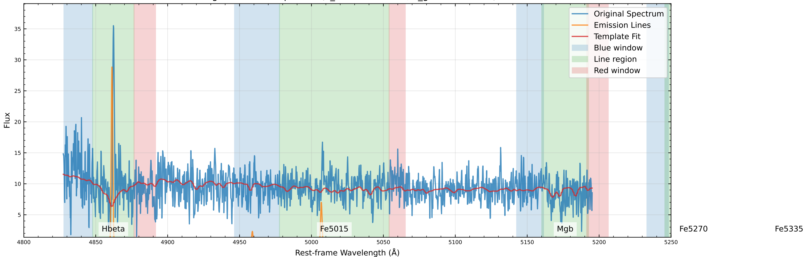
Original Data Comparison (v_star=41.6 km/s, v_gas=63.0 km/s)
