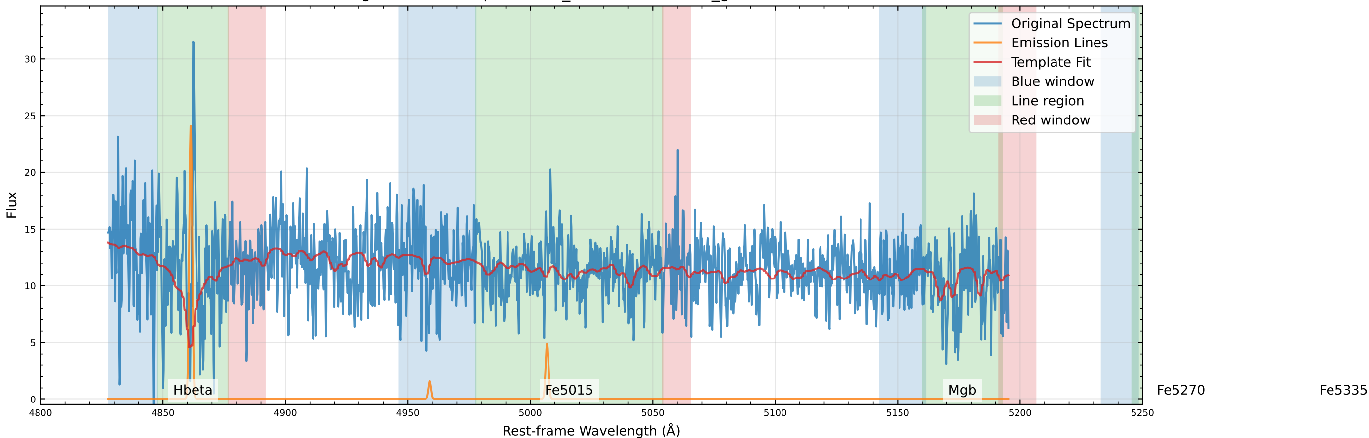
Original Data Comparison (v_star=88.0 km/s, v_gas=78.3 km/s)
