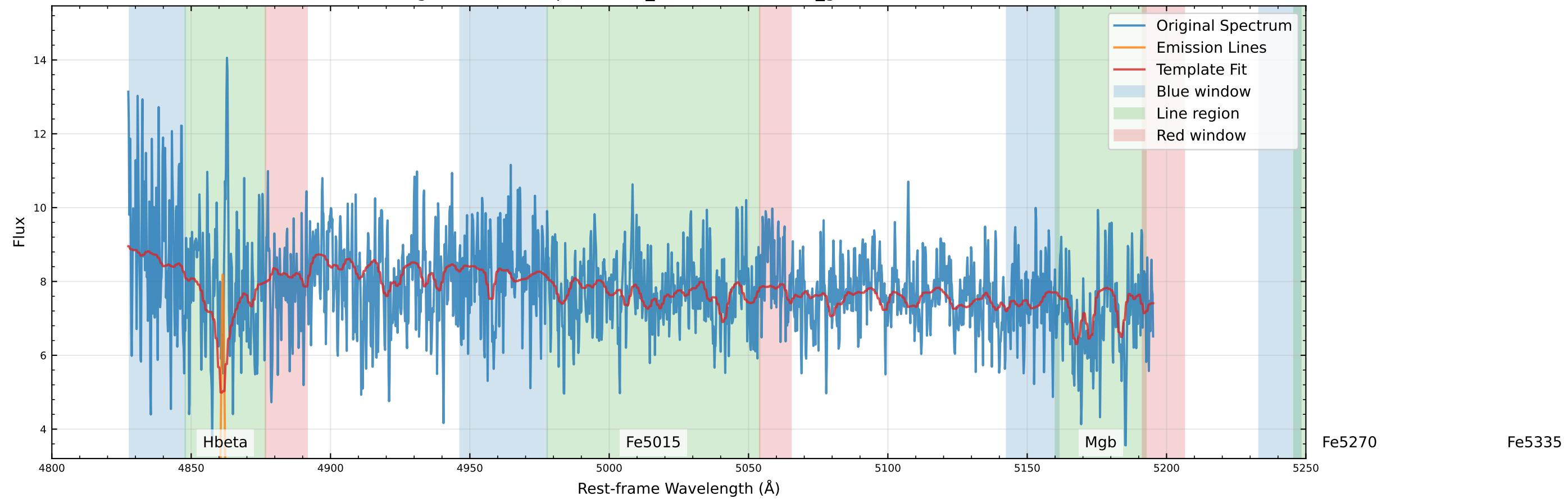
Original Data Comparison (v_star=72.9 km/s, v_gas=84.9 km/s)
