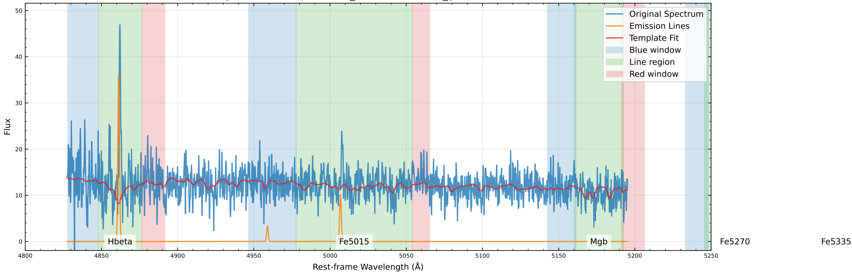
Original Data Comparison (v_star=43.5 km/s, v_gas=51.2 km/s)
