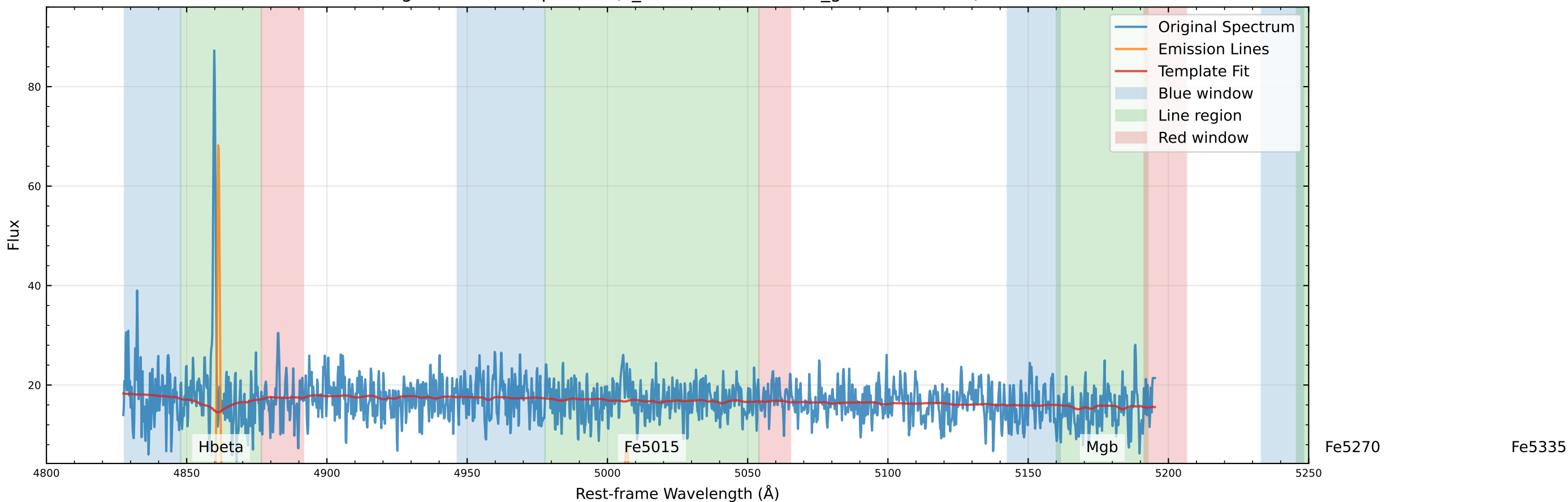
Original Data Comparison (v_star=-101.7 km/s, v_gas=-90.5 km/s)
