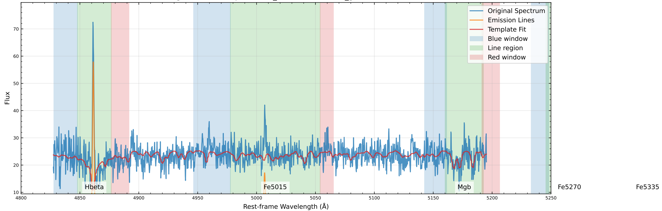
Original Data Comparison (v_star=17.7 km/s, v_gas=-2.2 km/s)
