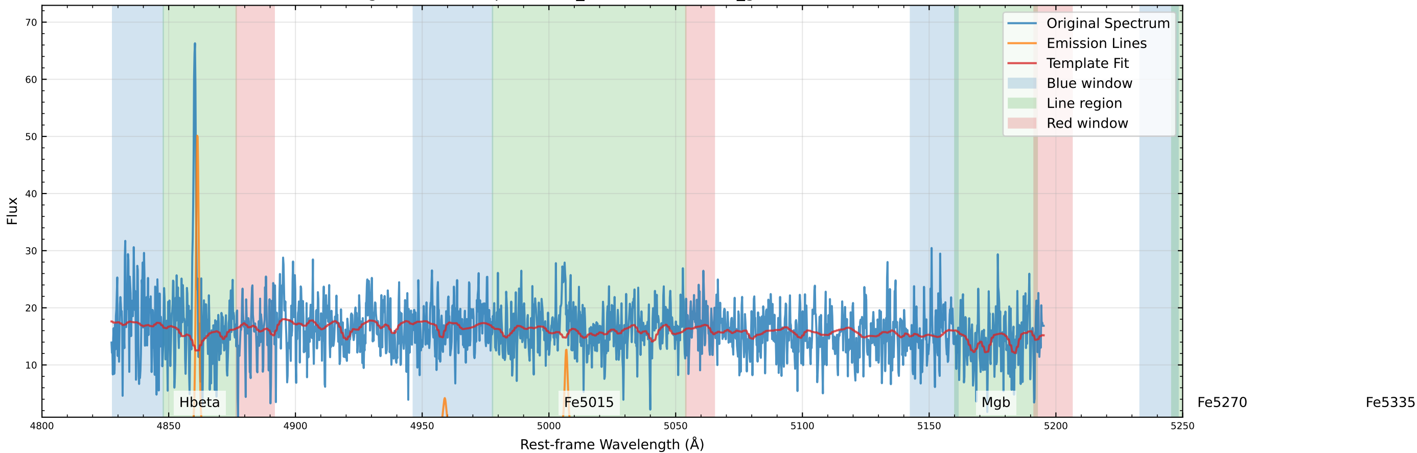
Original Data Comparison (v_star=-46.3 km/s, v_gas=-67.1 km/s)
